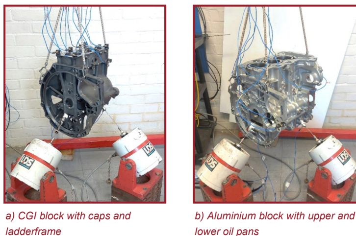
Figure 6: Experimental set-up for the NVH testing showing excitation shaker points on the flywheel end and on the lower side of the block, near the midpoint
